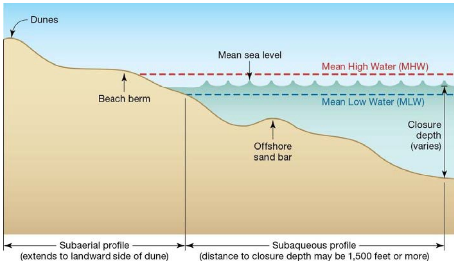
Figure 15. Typical Beach Profile
